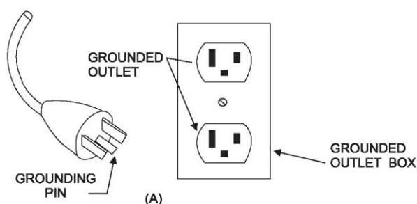
Grounding methods
